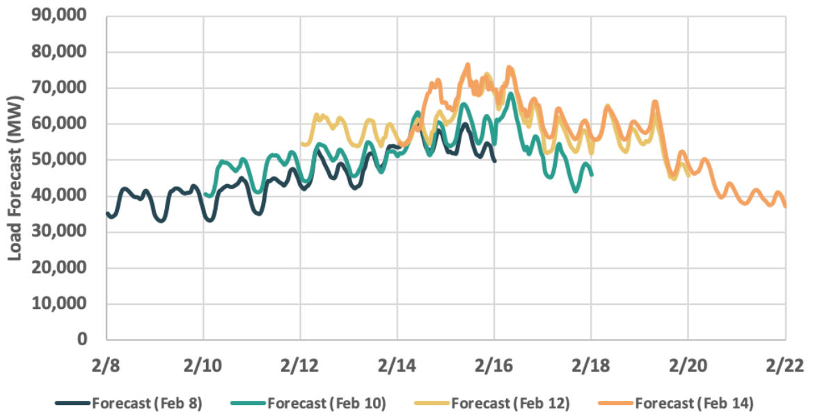
Figure 2.e. ERCOT 7-day (hourly resolution) load forecasts for February 8, 10, 12, and 14.
