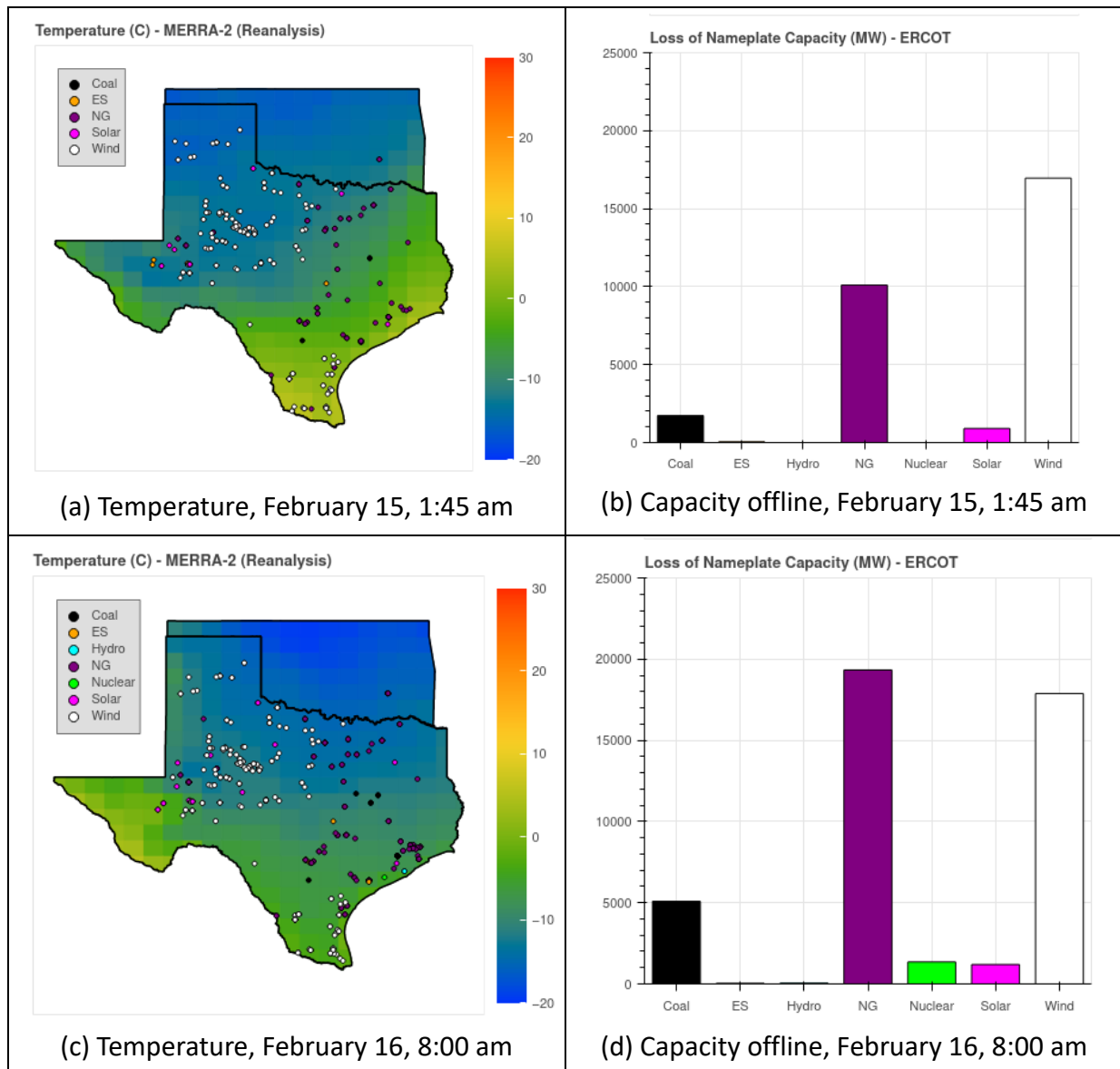
Figure 2.m. The temperature across Texas and reported loss of (nameplate) capacity by ERCOT for the critical time period of February 15, 1:45 a.m. (a and b) and the time of peak generation outage on February 16, 8:00 a.m. (c and d). 47
